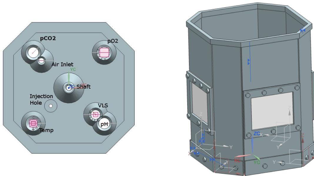
Figure: The phantom container (right) has four windows to place sensors of instruments. The distance between these windows is sufficient to avoid crosstalk between instruments. The container is filled with a solution of Intralipid®, human haemoglobin, buffer, glucose, salt (physiological concentration) and yeast. The solutions is constantly stirred and kept at 37°C. The lid (left) is an airtight cover to achieve equilibrium of the gases in the solution quickly. It allows the placement of different sensors to measure temperature, pH, pCO 2 , and take or inset samples.
