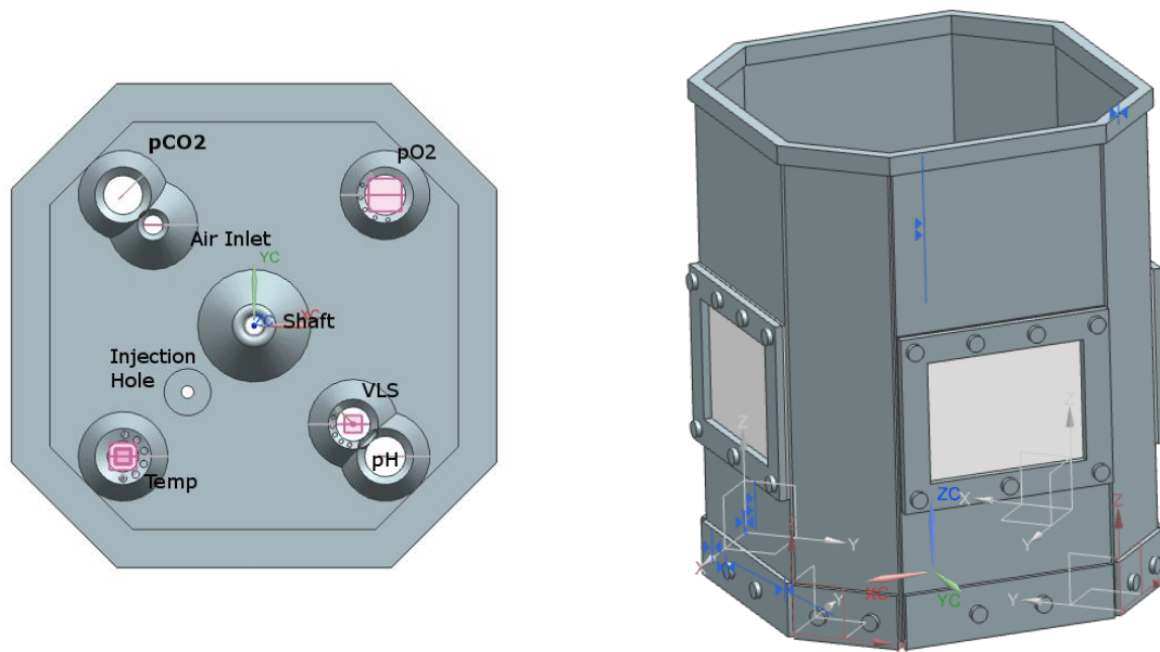
Figure: The phantom container (right) has four windows to place sensors of instruments. The distance between these windows is sufficient to avoid crosstalk between instruments. The container is filled with a solution of Intralipid®, human haemoglobin, buffer, glucose, salt (physiological concentration) and yeast. The solution is constantly stirred and kept at 37°C. The lid (left) is an airtight cover to achieve equilibrium of the gases in the solution quickly. It allows the placement of different sensors to measure temperature, pH, pCO 2 , and take or inset samples.
